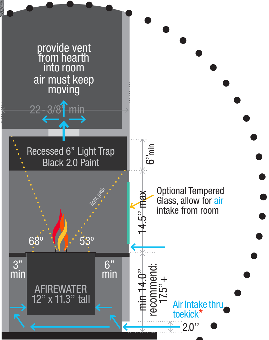
SIDE SECTION SCHEMATIC GLASS ENCLOSED RECESSED HEARTH
